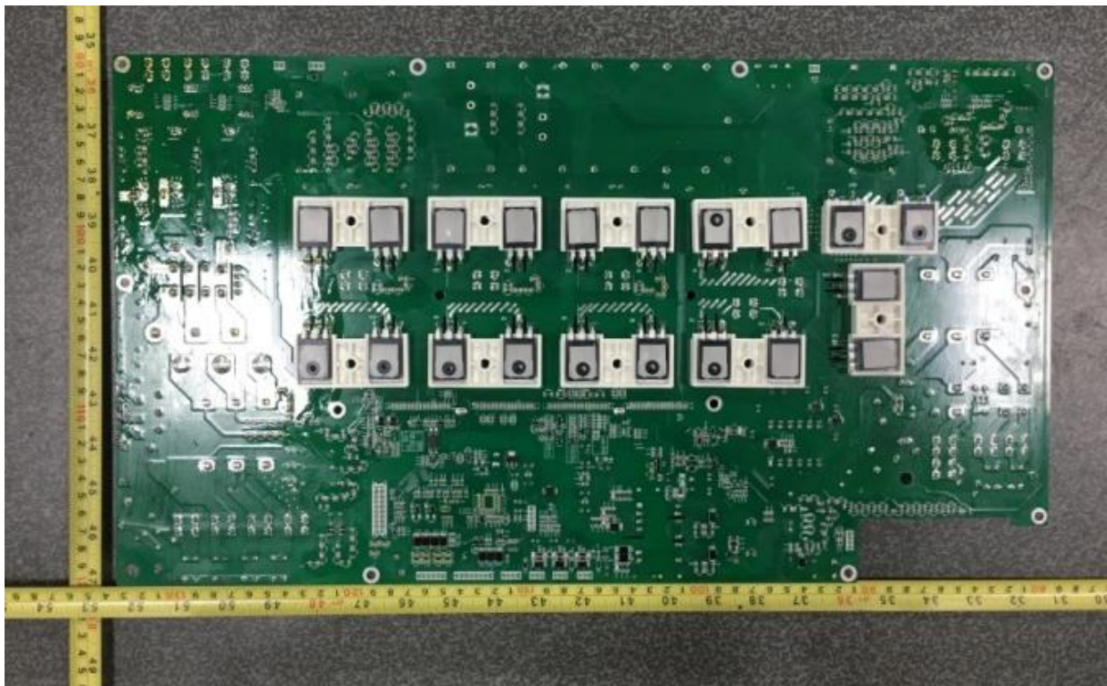
Figure 8 Power board solder side view
