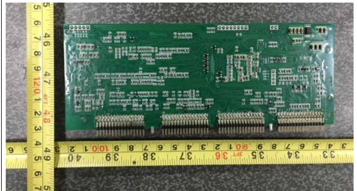
Figure 12 Control power board solder side view
