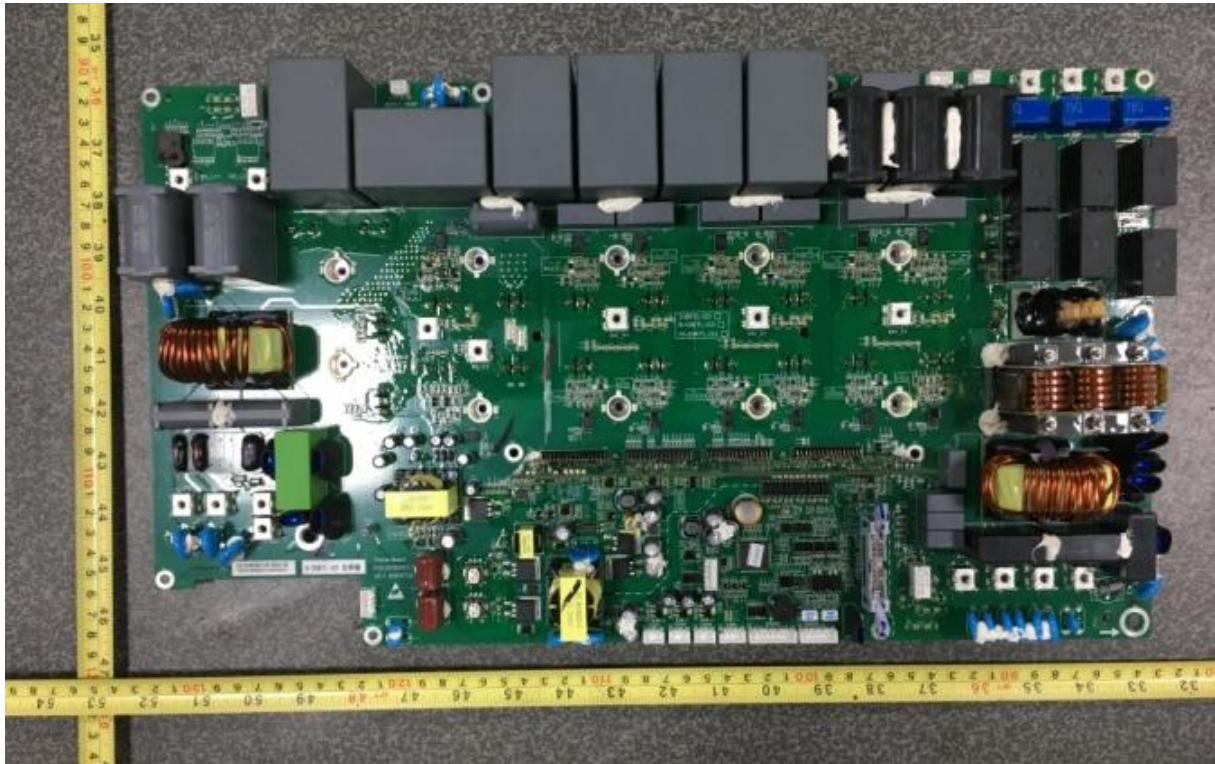
Figure 7 Power board component side view
