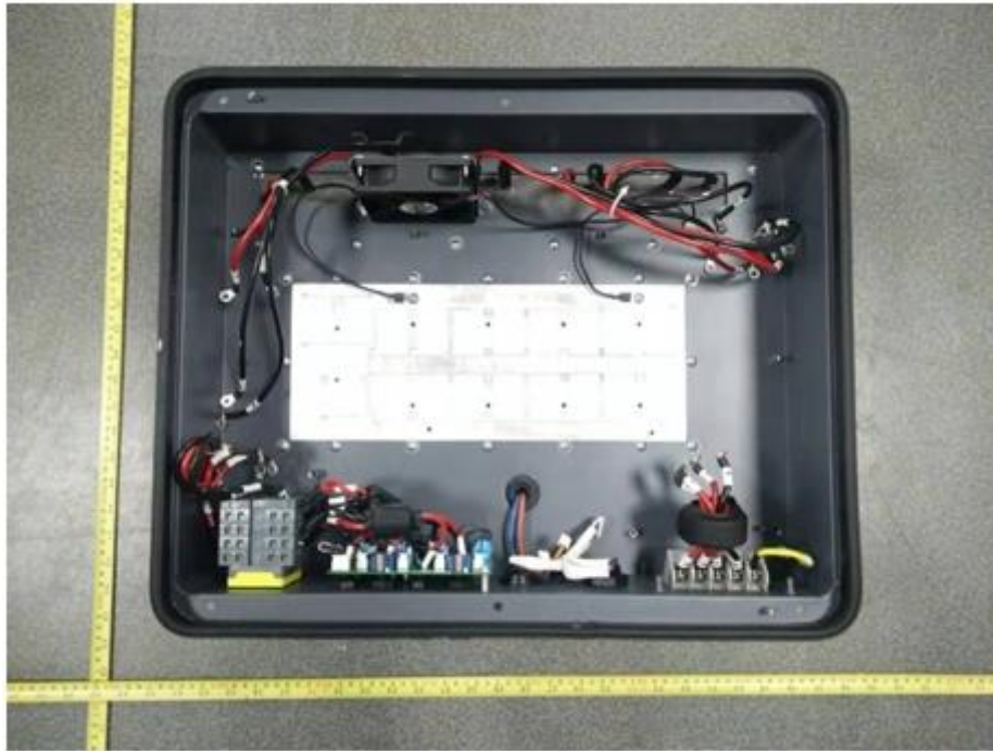
Figure 13 Internal view
